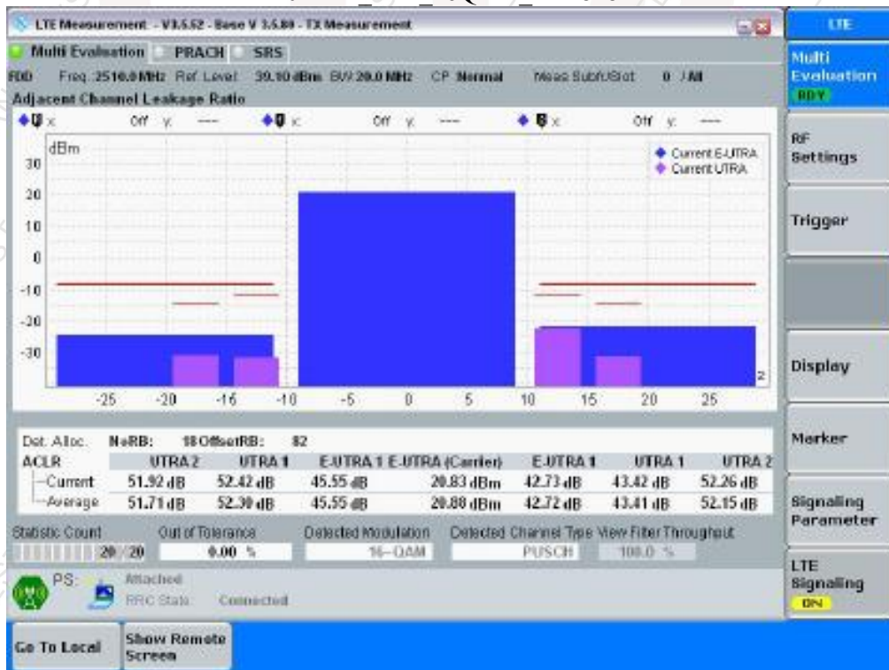
20 MHz Low 16QAM RB18#82
