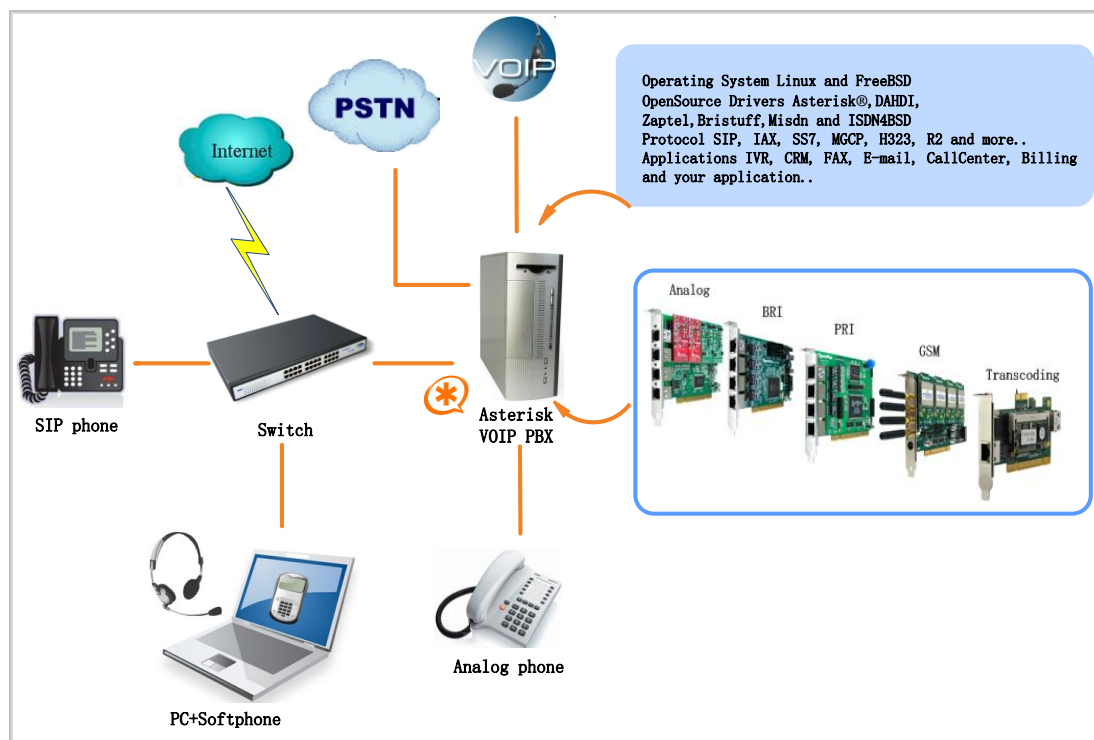
Figure 1 Topology
