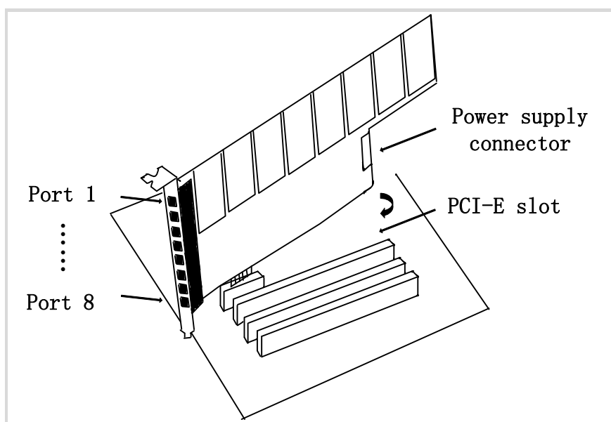
Figure 4 Hardware setup
