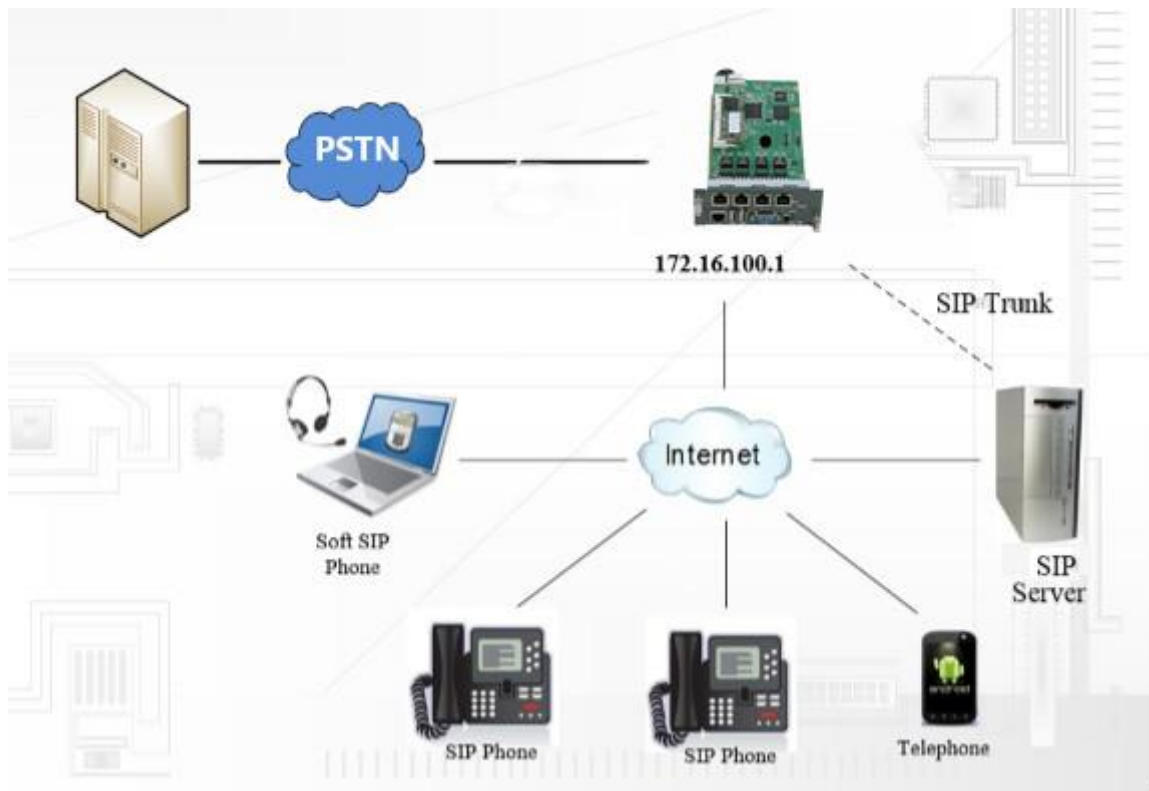
Figure 1-2-1 Topological Graph
