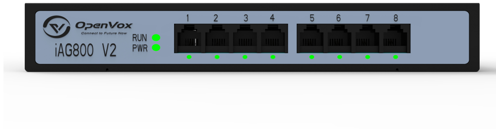
Figure 1-3-2 Front Panel
