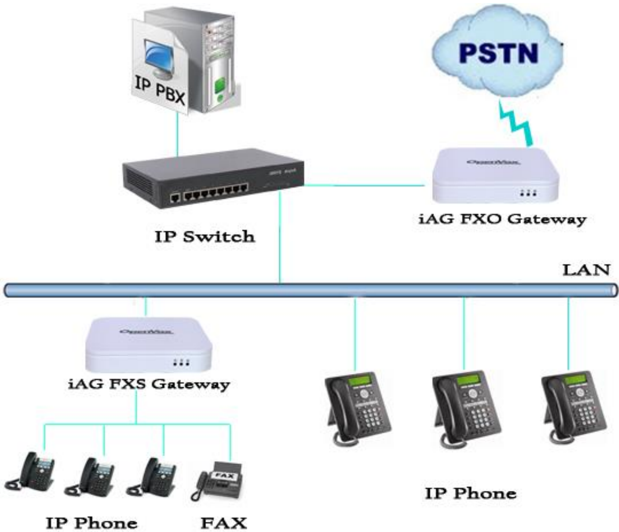
Figure 1-2-1 Topological Graph
